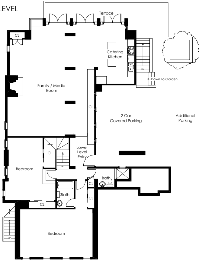
MAIN LEVEL
