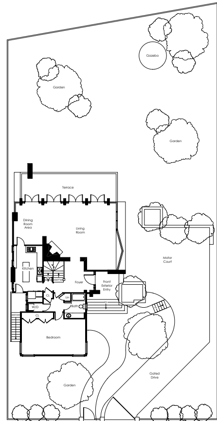
PLOT PLAN
